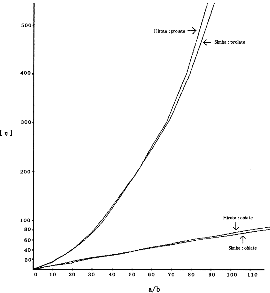
FIGURE 4 Relationship of nondimensional intrinsic viscosity, [\eta] , to the axial ratio, a/b , of an ellipsoid.
